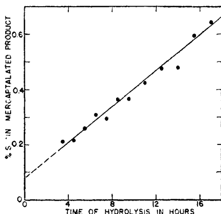
FIG. 5. Hydrolysis of methylated cellulose in fuming hydrochloric acid at 0°C. Reaction followed by mercaptalation method. (Wolfrom, Sowden, and Lassetre (92).)
