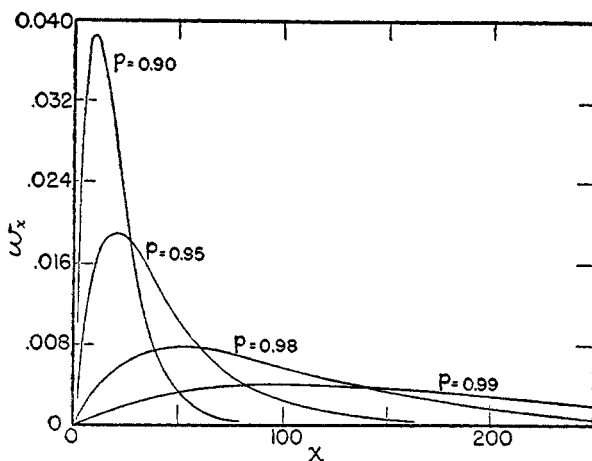
FIG. 9. Molecular-weight distributions for linear condensation polymers on a weight basis for several values of the extent of reaction p . Weight fractions w_x vs. number of structural units, x , as calculated from equation 10. See reference 27.
